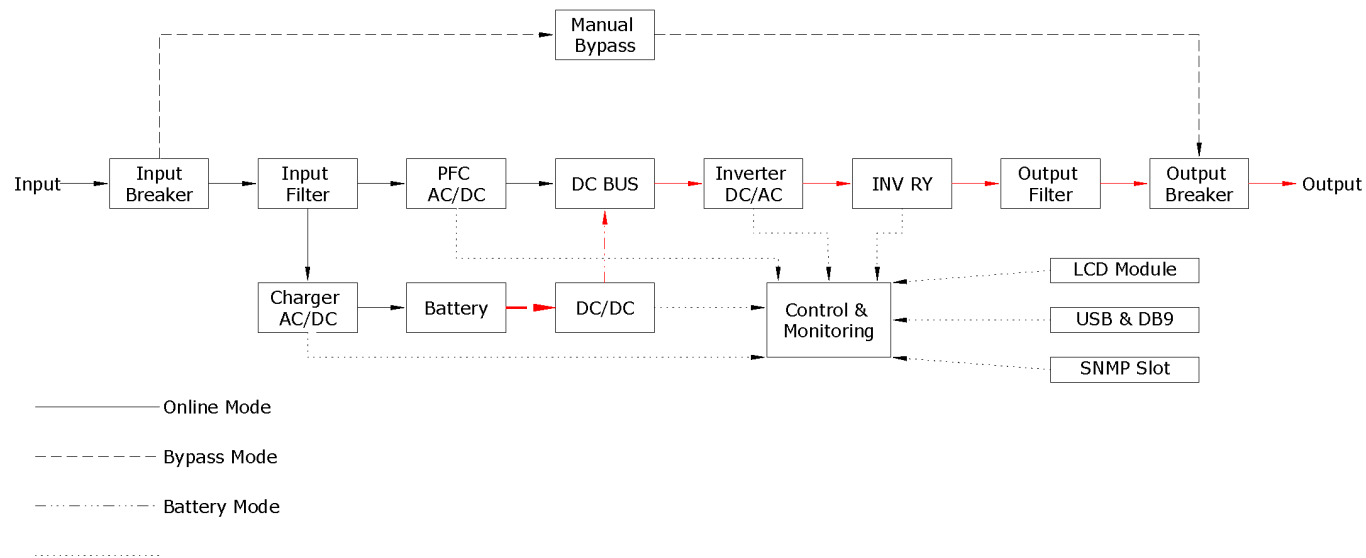
Figure 4 Single Line Drawing - Battery Operation
