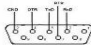
View Facing Outside of DB9 Female Connector
