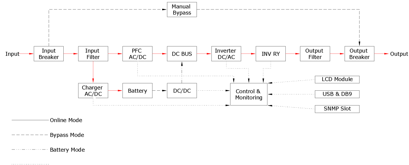
Figure 2 Single Line Drawing - Normal Operation
